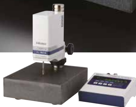
Losse meetunit VL-50S-B
