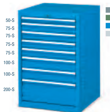
•ORD. NO. DRAWERS F DD 1075 54 04 8 Cabinet with 8 normal extension drawers Dimensions mm 564x726x850 h Central lock
