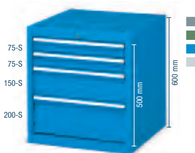
ORD. NO. DRAWERS F DD 1050 52 04 4 Cabinet with 4 normal extension drawers Dim. mm 564x726x600 h Central lock
