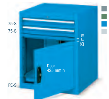
• ORD. NO. DRAWERS F DD 1160 51 04 2 Cabinet with 2 normal extension drawers 1 normal retractable shelf Dim. mm 564x726x700 h Central lock
