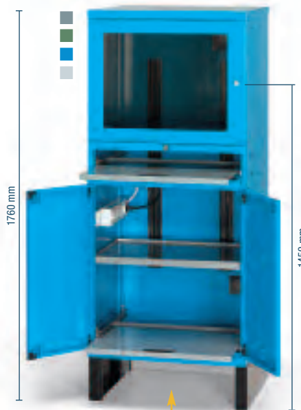
Dim. mm 717x635x1760 h Complete with: 2 height adjustable shelves 1 retractable keyboard shelf 1 retractable shelf 1 pair of 200 mm h base plinths without facing piece
