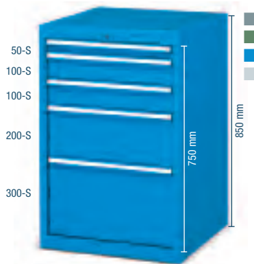
•ORD. NO. DRAWERS F DD 1075 51 04 5 Cabinet with 5 normal extension drawers Dim. mm 564x726x850 h Central lock
